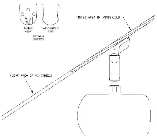
Figure 2.3d Proper antenna mounting.
