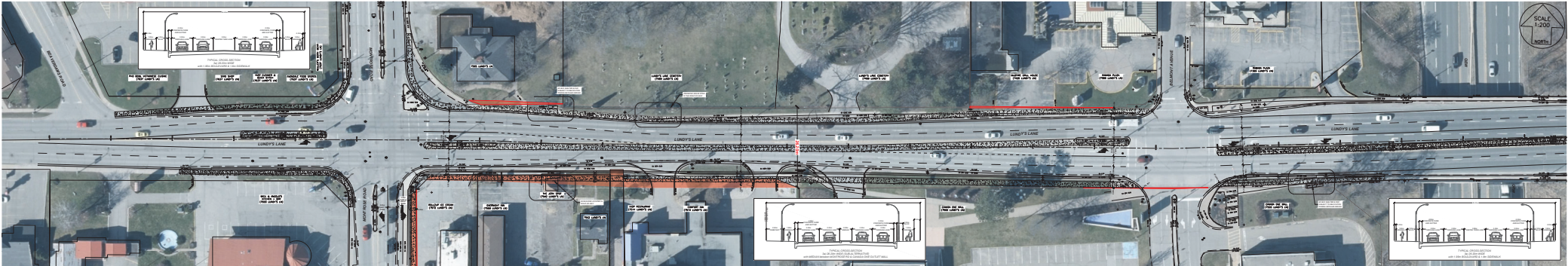
PR 26.20m RIGHT-OF-WAY PREFERRED ALTERNATIVE 3A (SUB-ALTERNATIVE BETWEEN MONTROSE RD & CANADA ONE OUTLET MALL)
