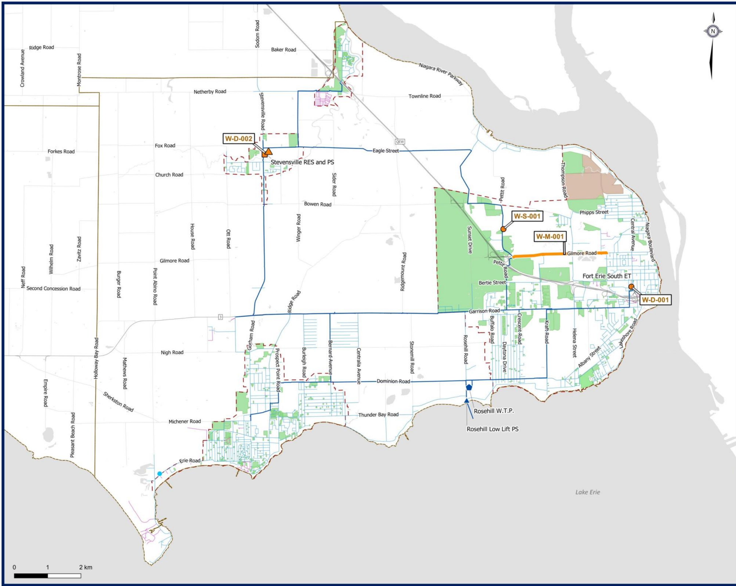
Figure 3.D.14 Fort Erie Preferred Water Servicing Strategy
