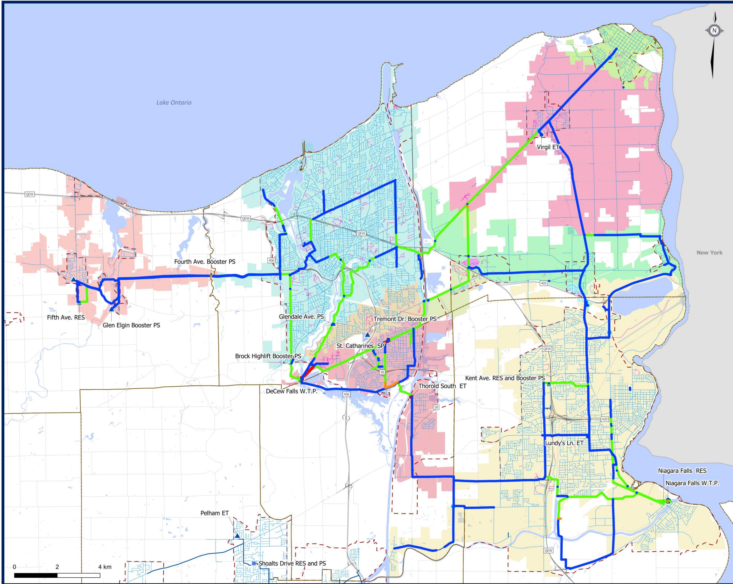
Figure 3.C.12 DeCew and Niagara Falls System 2051 System Watermain Velocity
