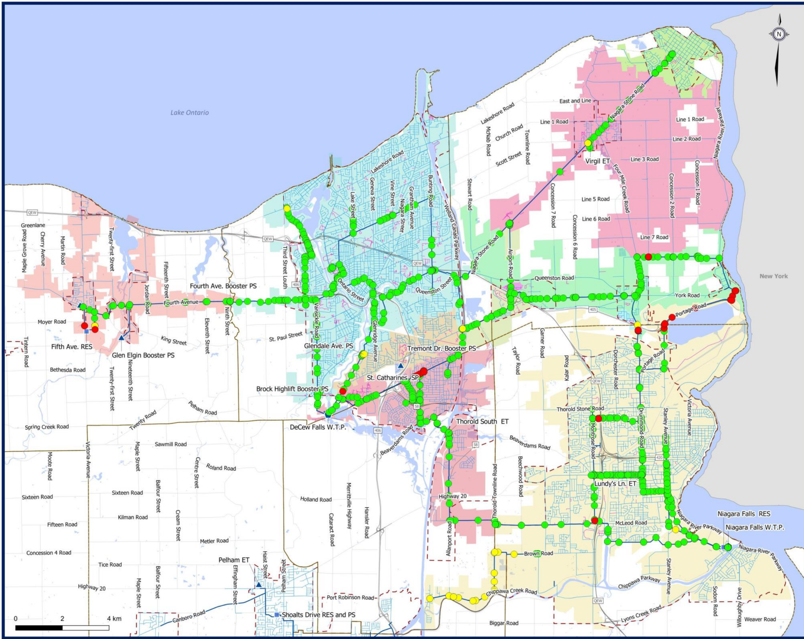
Figure 3.B.5 DeCew Falls System Existing System Fire Flows
