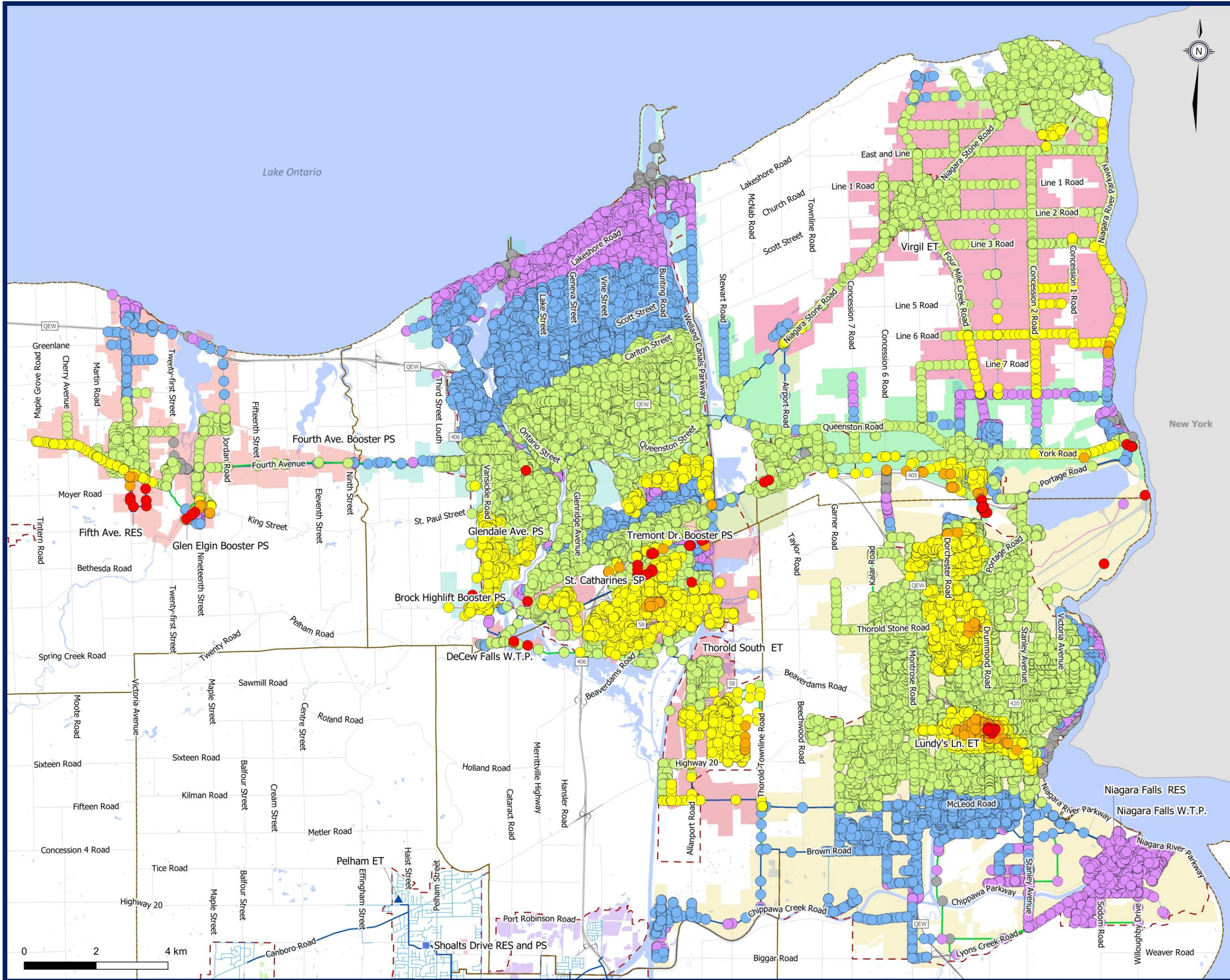
Figure 3.C.9 DeCew and Niagara Falls System 2051 System Peak Hour Pressures
