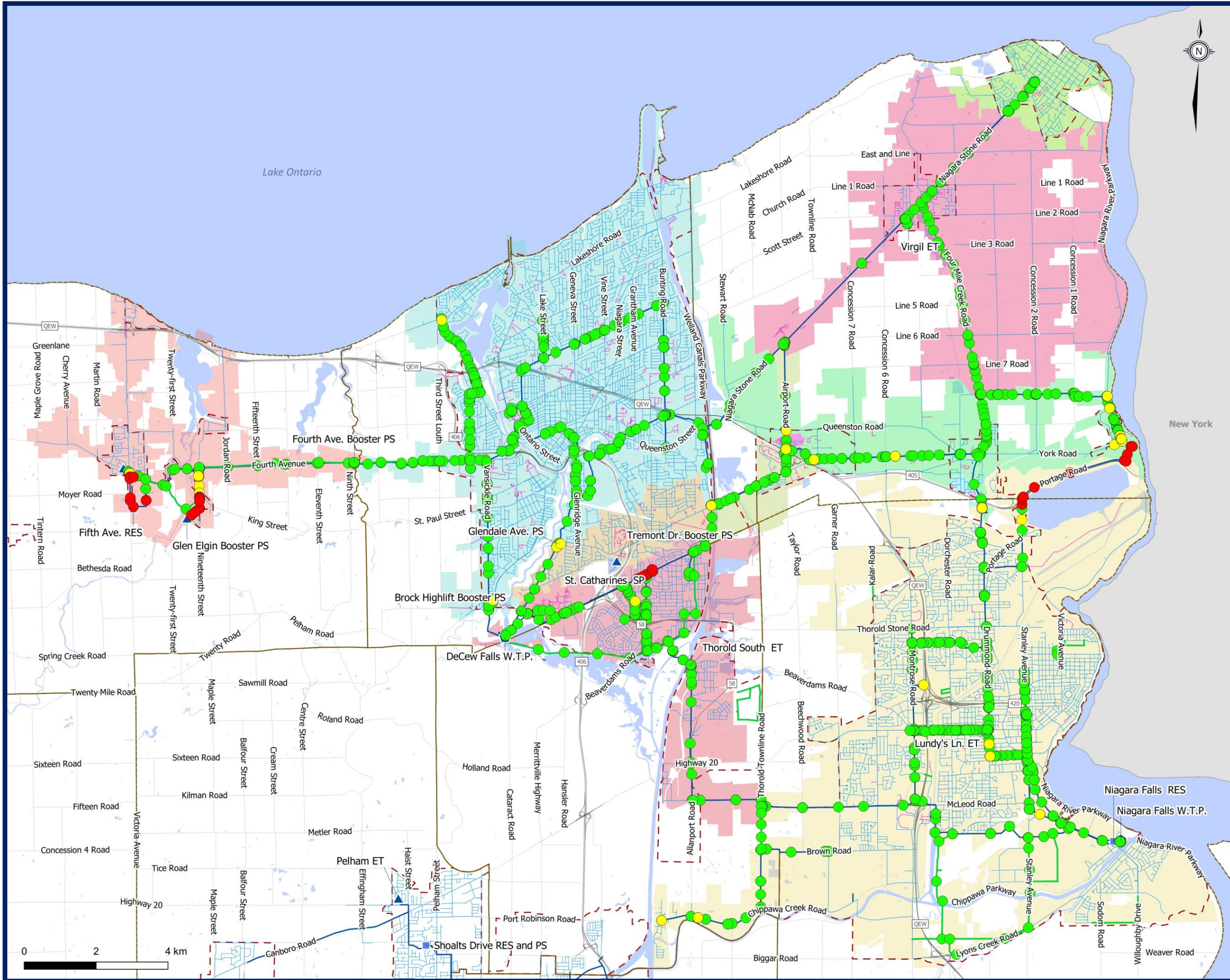
Figure 3.C.10 DeCew and Niagara Falls System 2051 System Fire Flows
