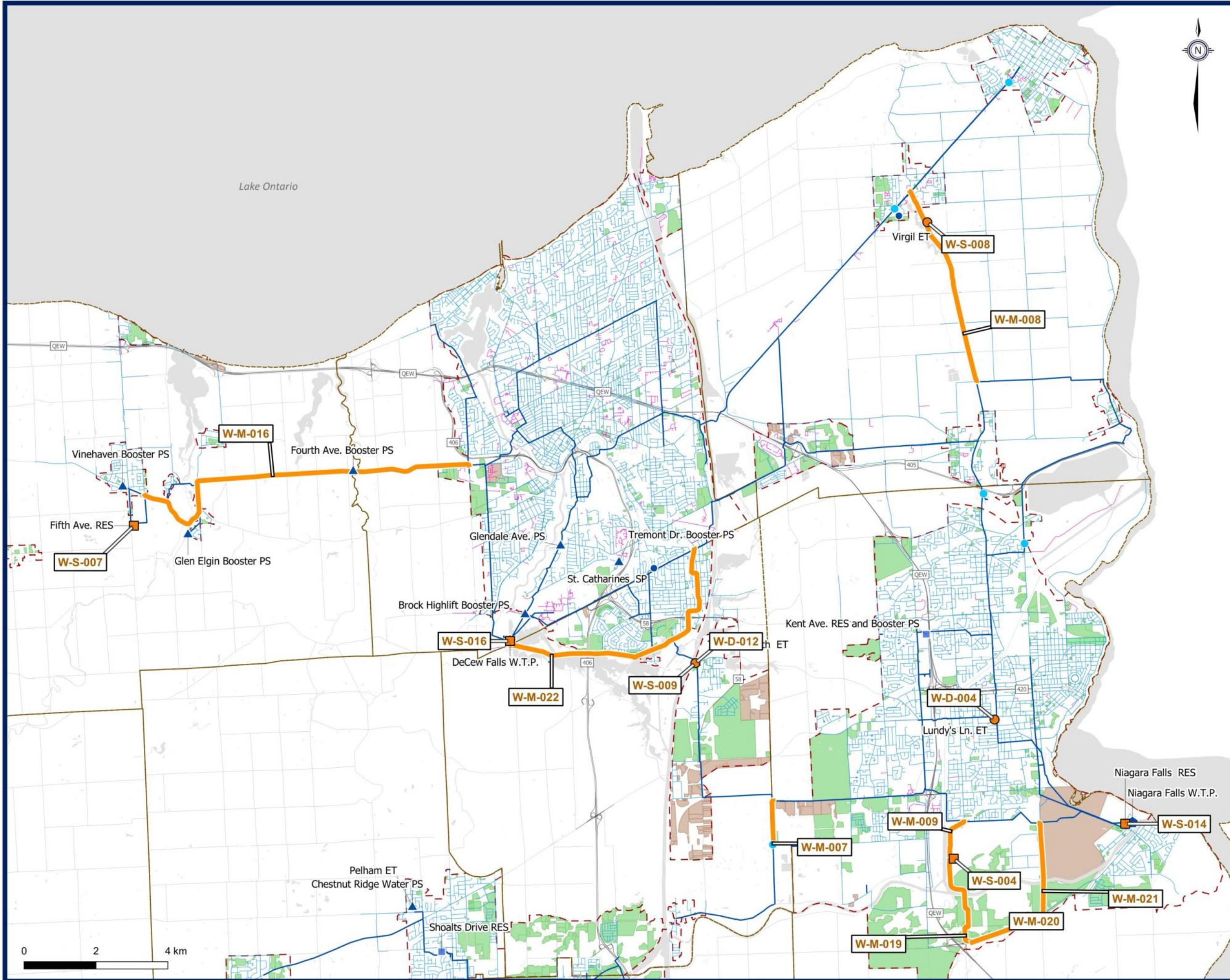
Figure 3.B.17 DeCew Falls System Preferred Water Servicing Strategy
