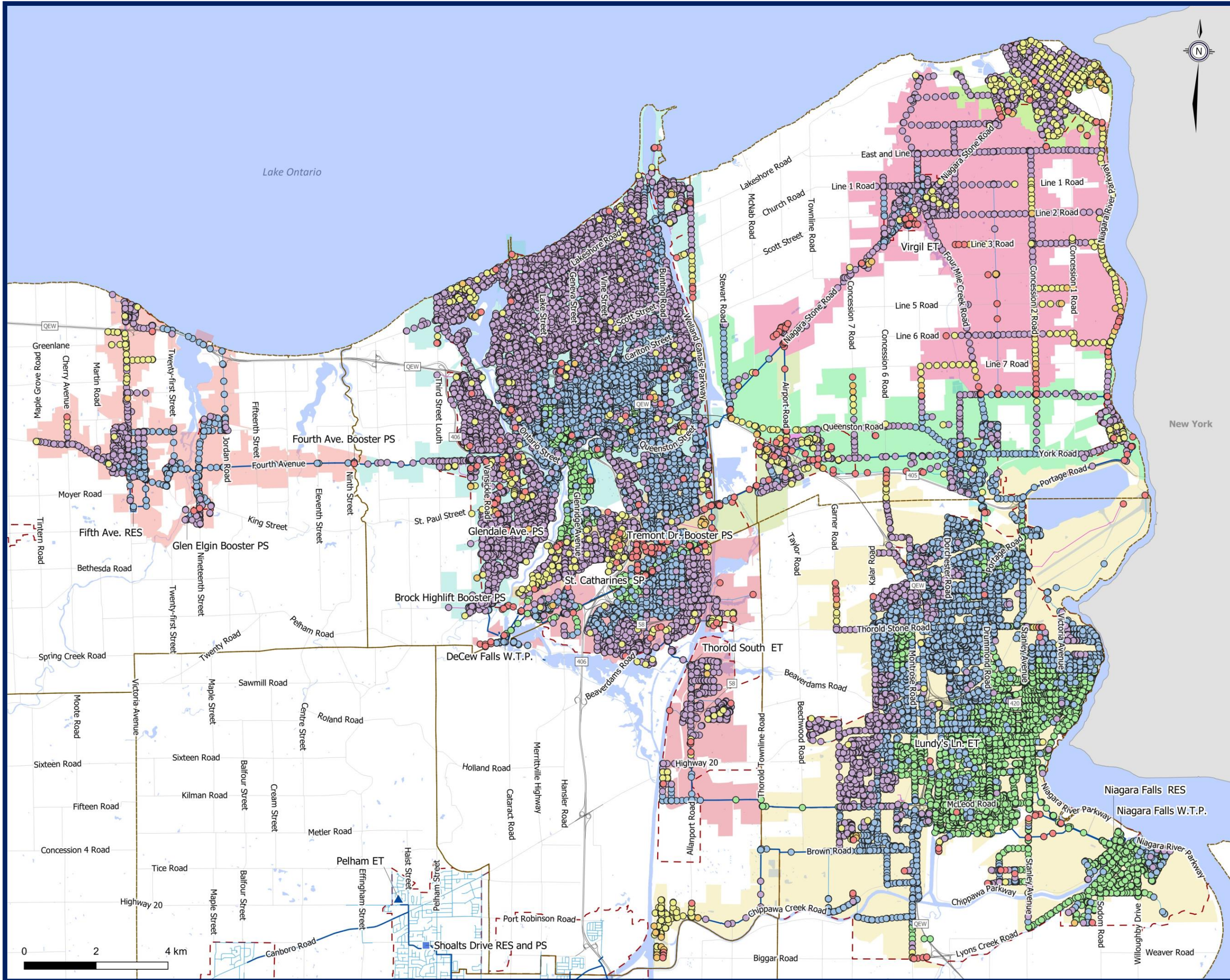
Figure 3.C.6 DeCew and Niagara Falls System Existing System Water Age
