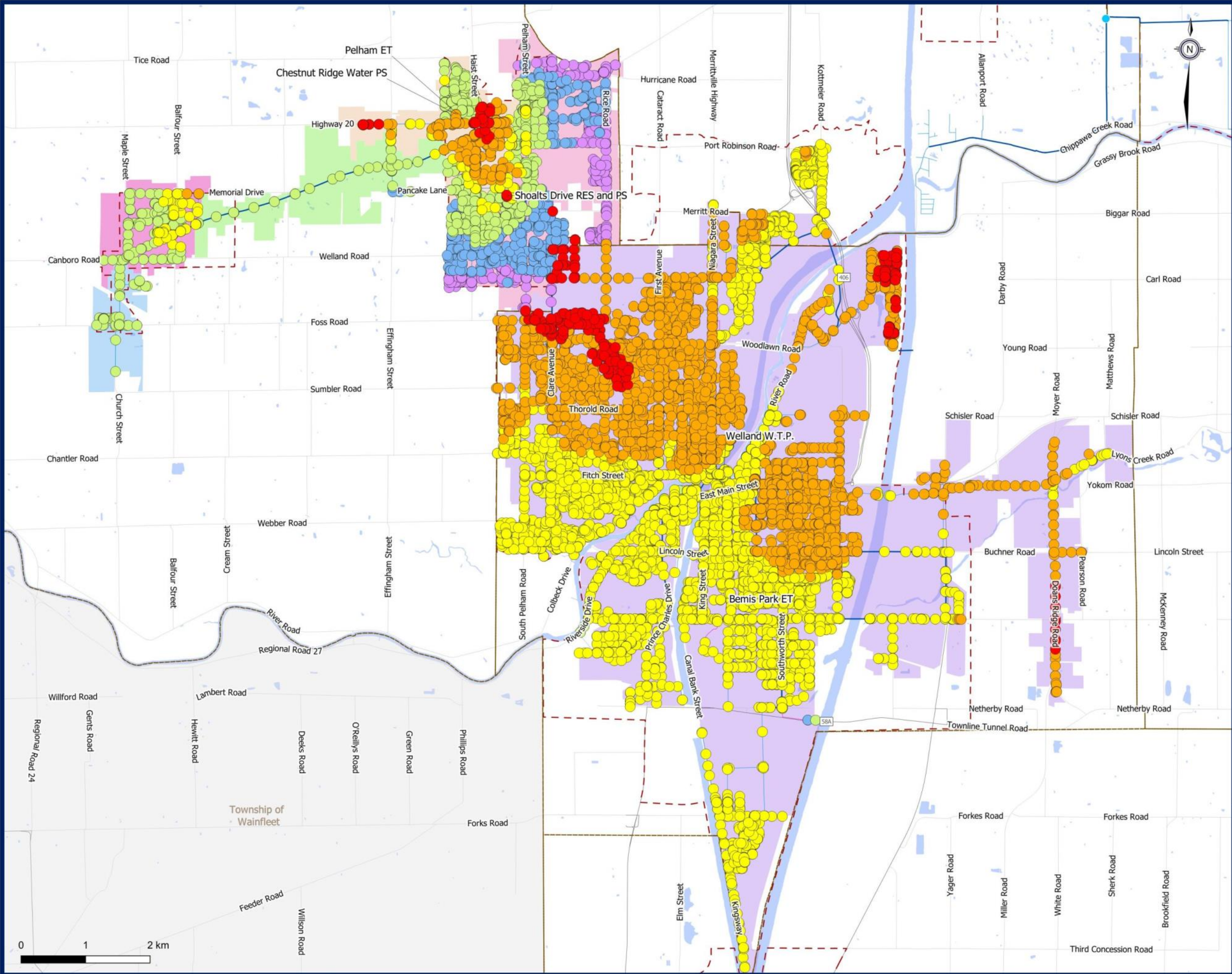
Figure 3.F.4 Welland Existing System Peak Hour Pressures
