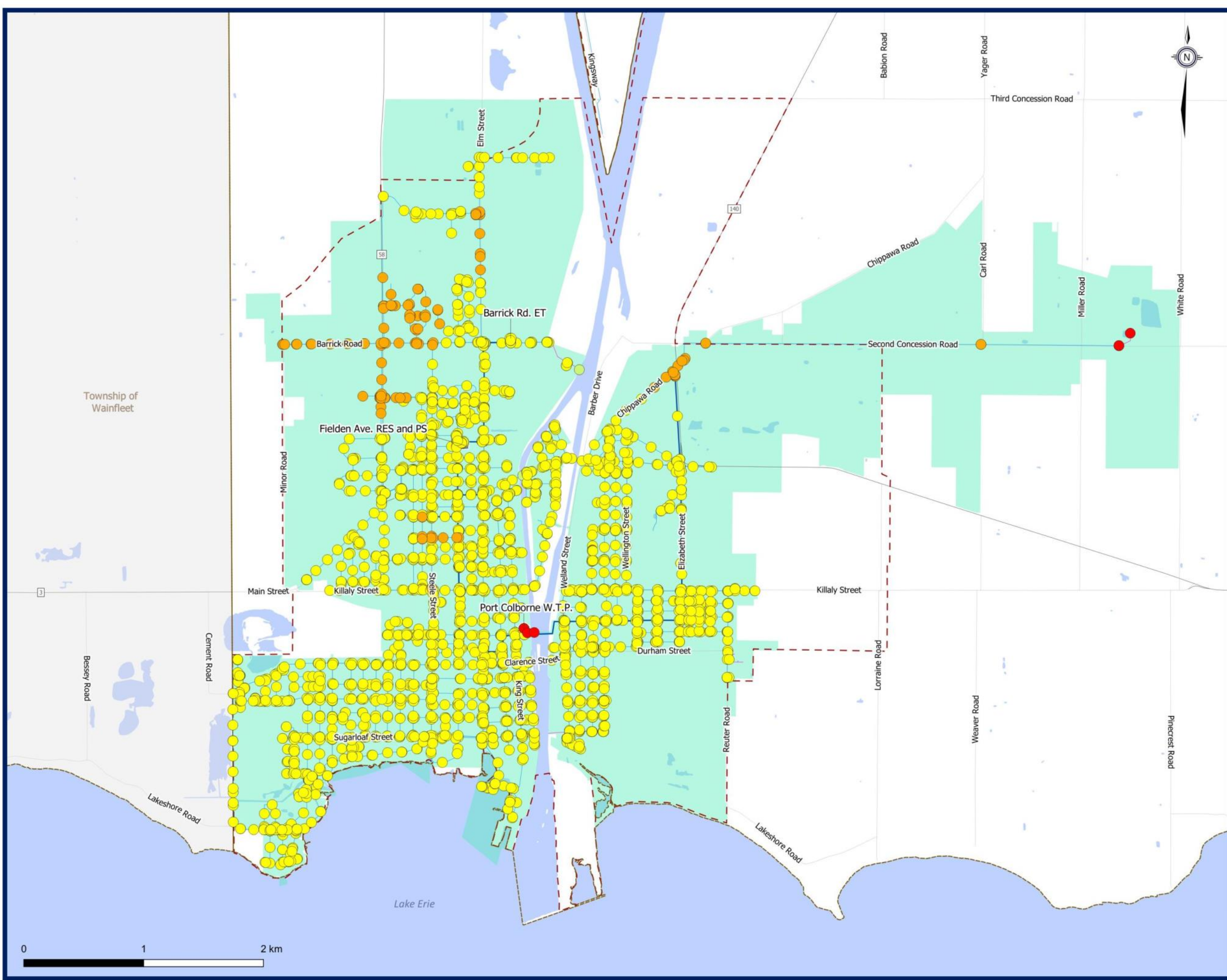
Figure 3.E.4 Port Colborne Existing System Peak Hour Pressures
