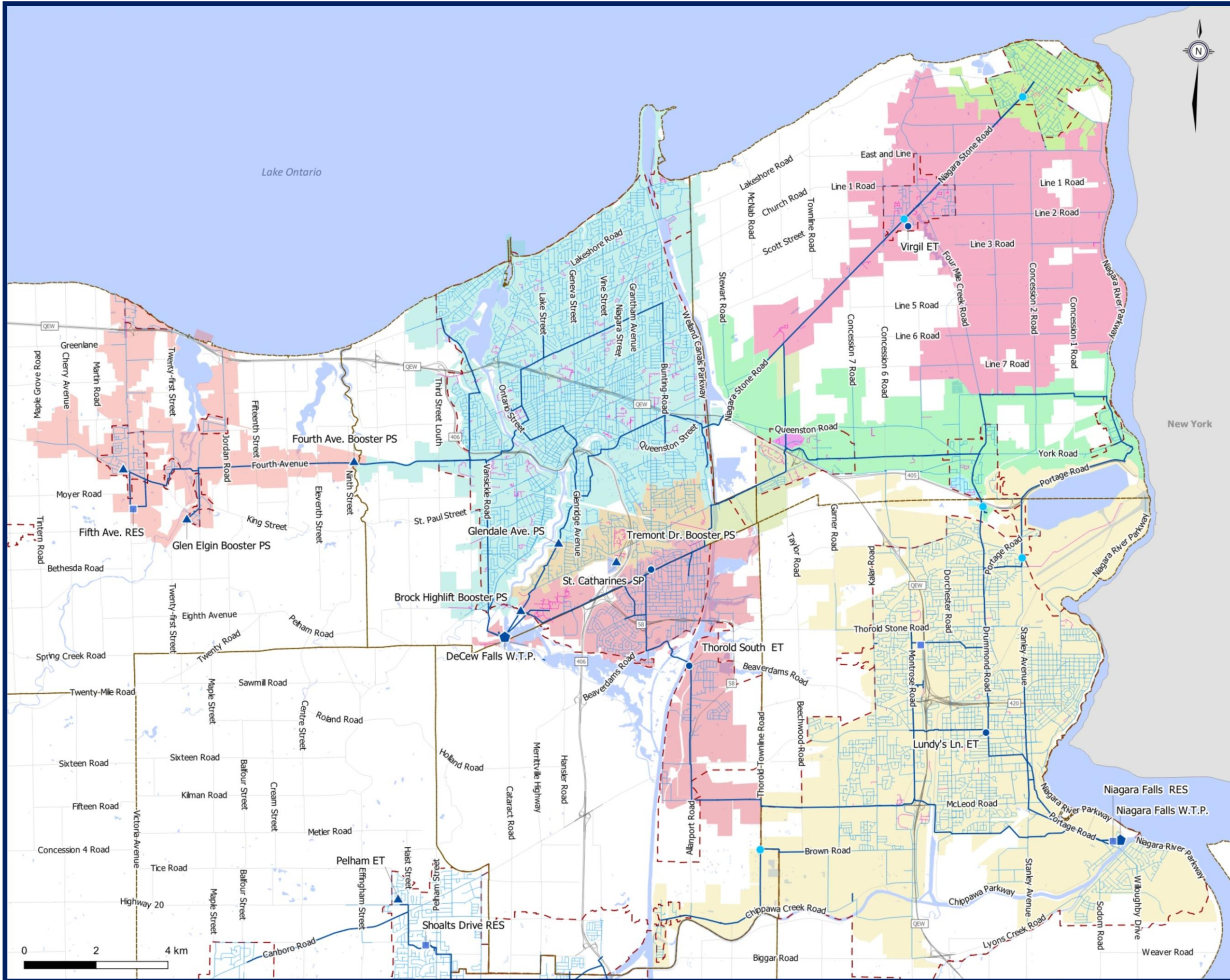
Figure 3.C.1 DeCew and Niagara Falls System Existing Water Infrastructure
