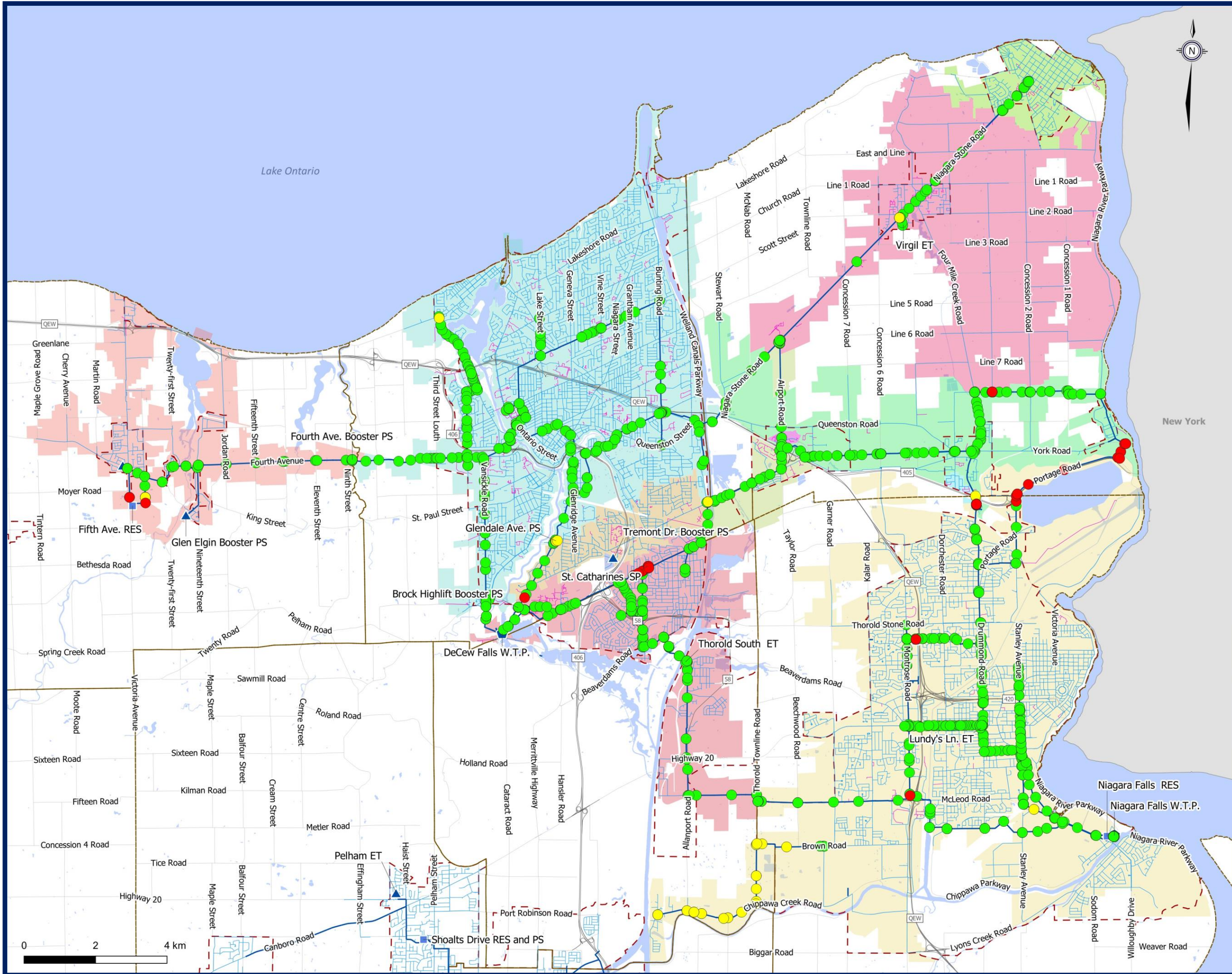
Figure 3.C.5 DeCew and Niagara Falls System Existing System Fire Flows
