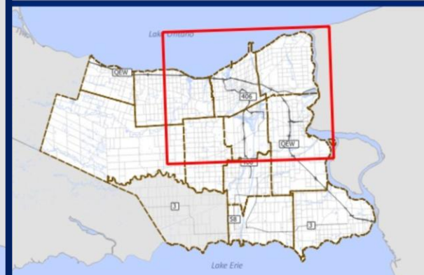
Figure 3.C.1 DeCew and Niagara Falls System Existing Water Infrastructure
