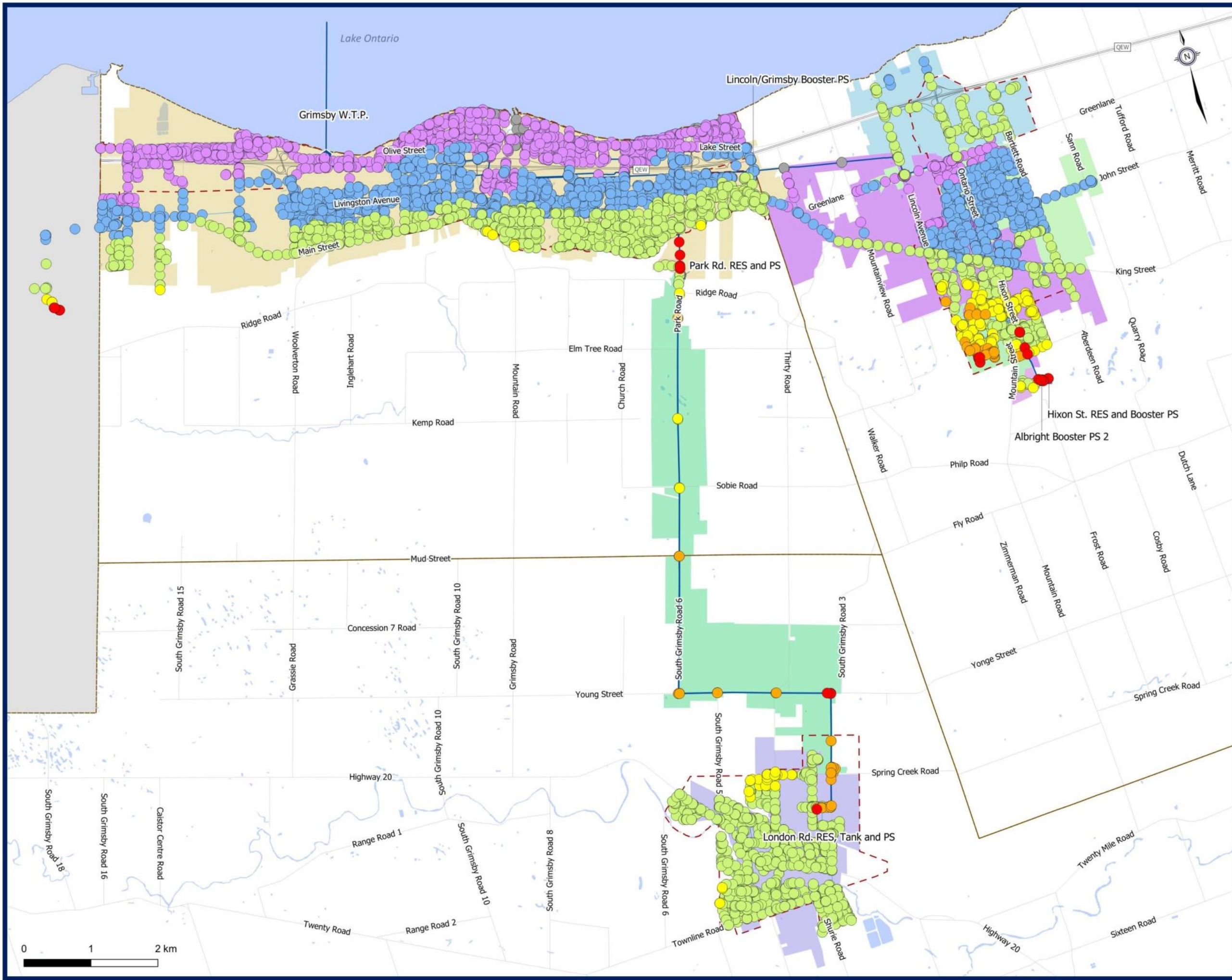
Figure 3.A.4 Grimsby System Existing System Peak Hour Pressures
