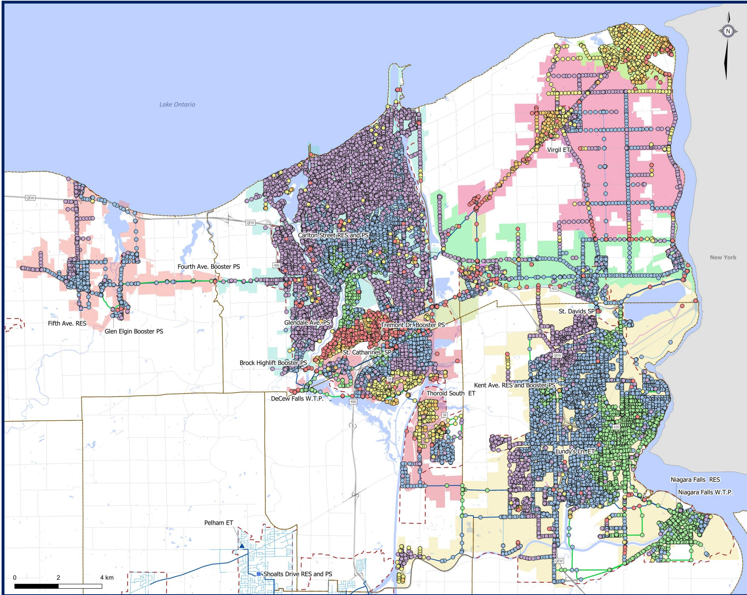
Figure 3.C.11 DeCew and Niagara Falls System 2051 System Water Age
