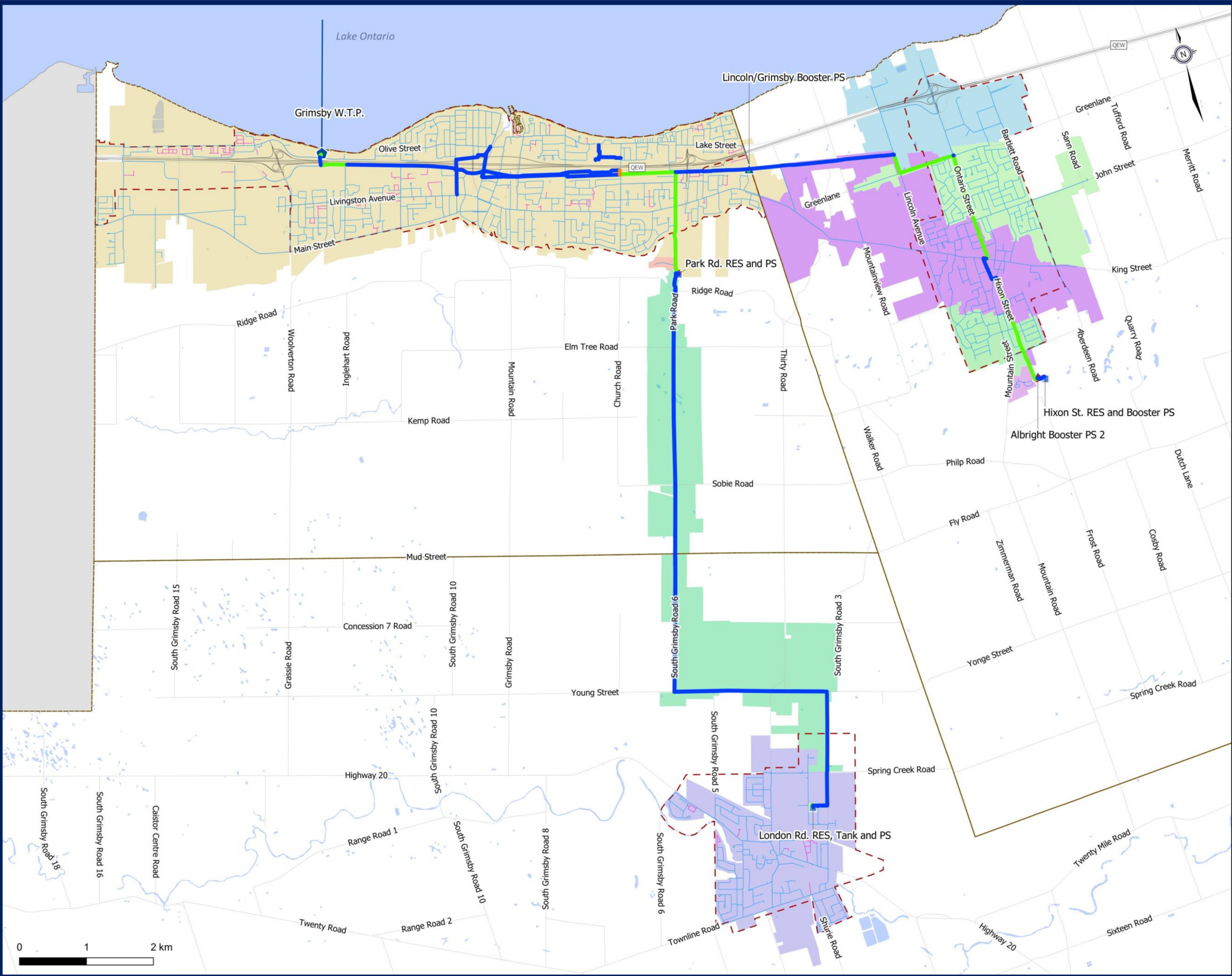
Existing System Watermain Velocity
