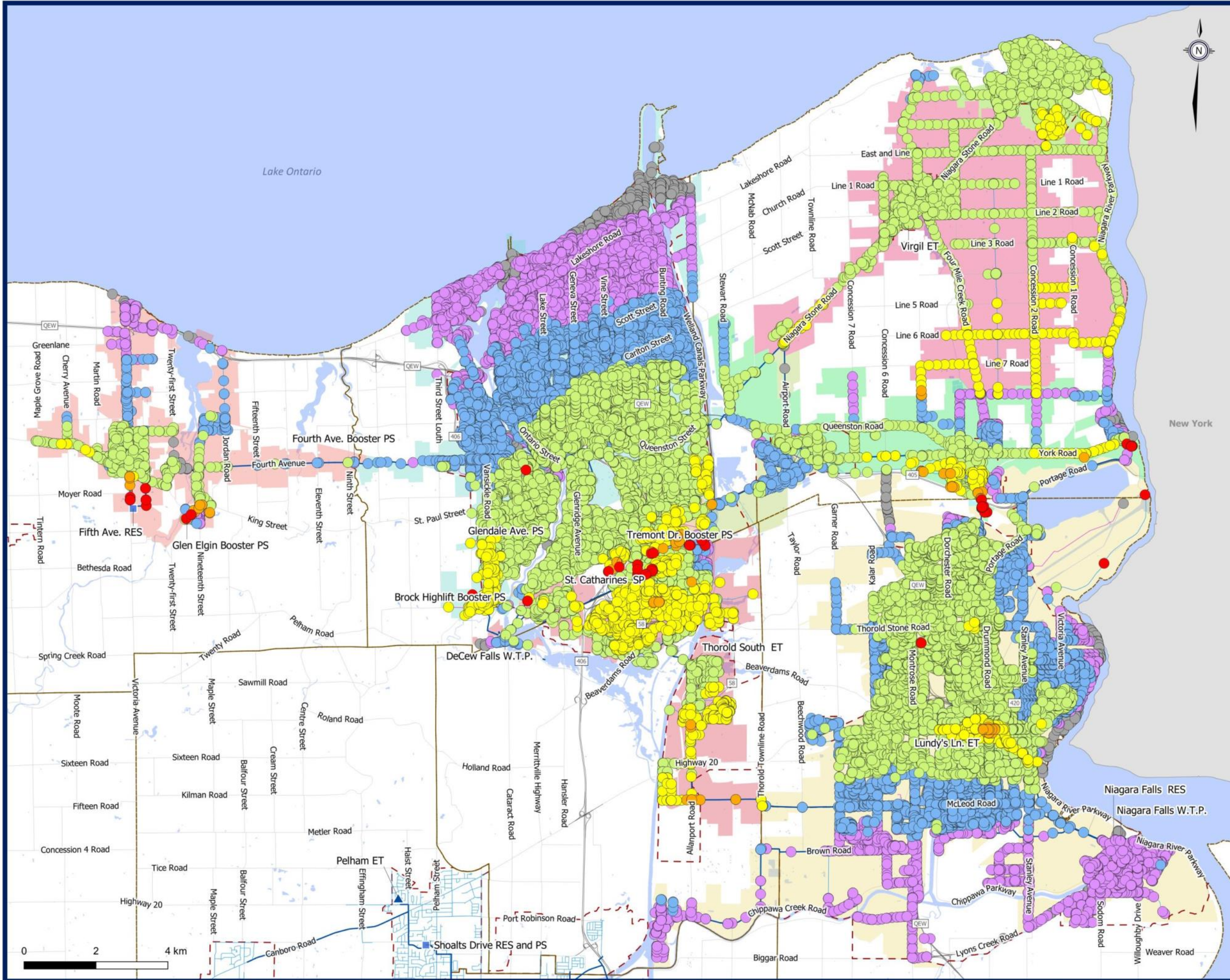
Figure 3.B.4 DeCew Falls System Existing System Peak Hour Pressures
