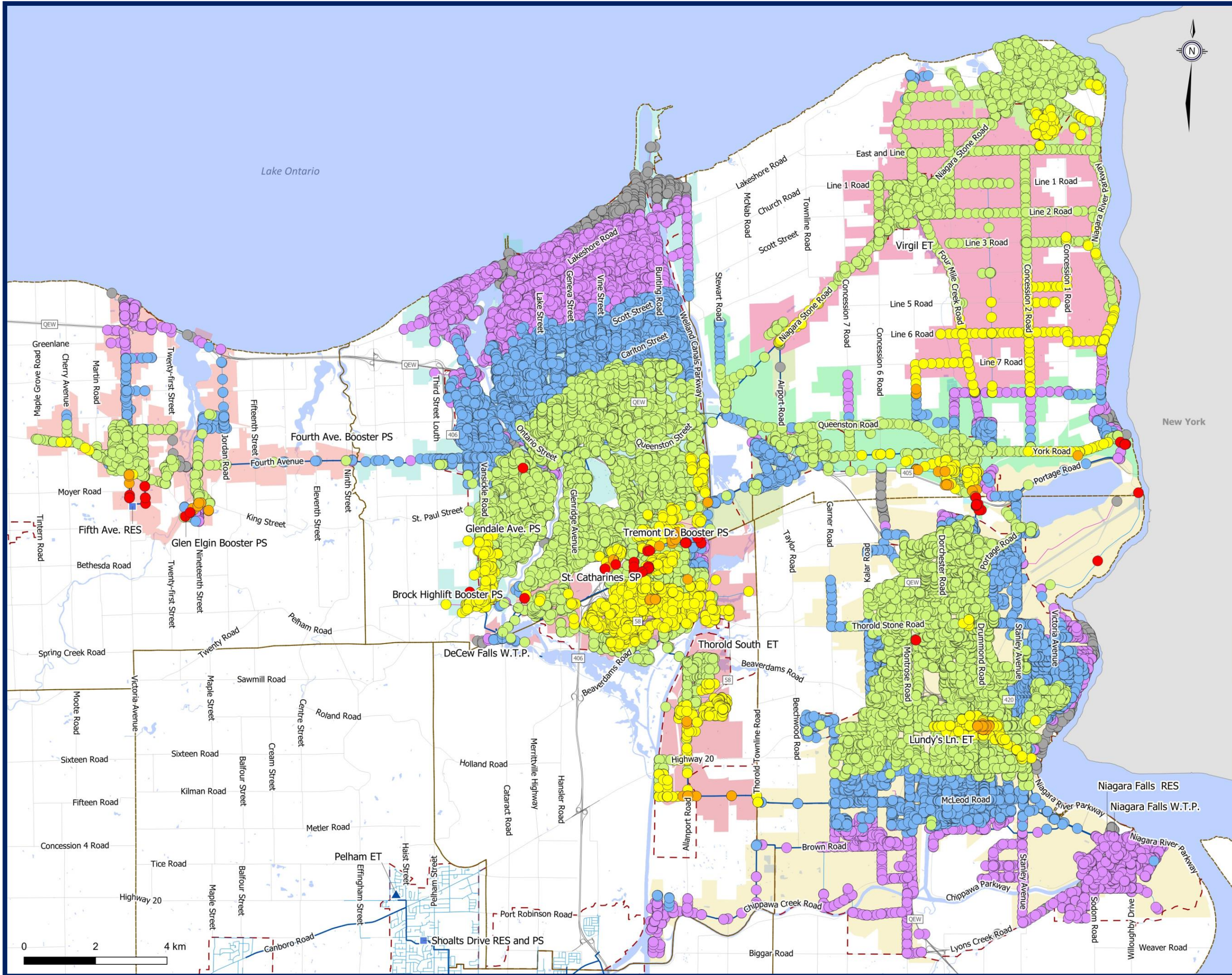
Figure 3.C.4 DeCew and Niagara Falls System Existing System Peak Hour Pressures
