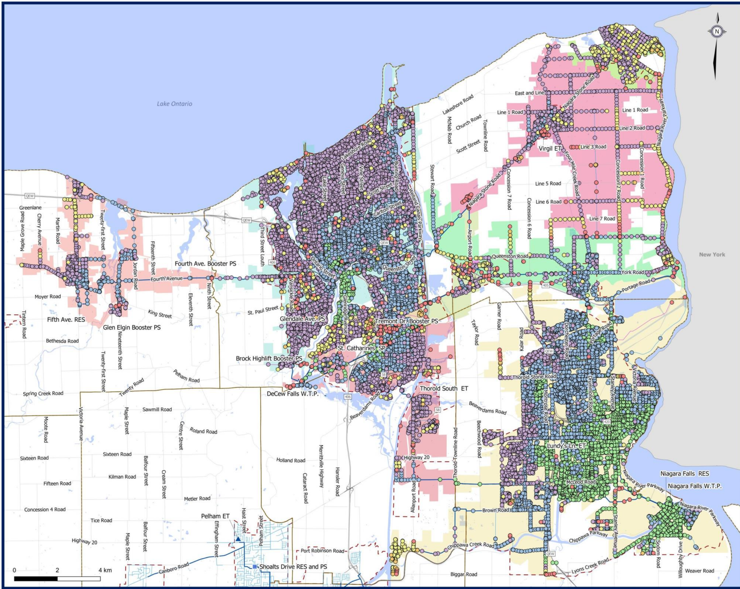
Figure 3.B.6 DeCew Falls System Existing System Water Age
