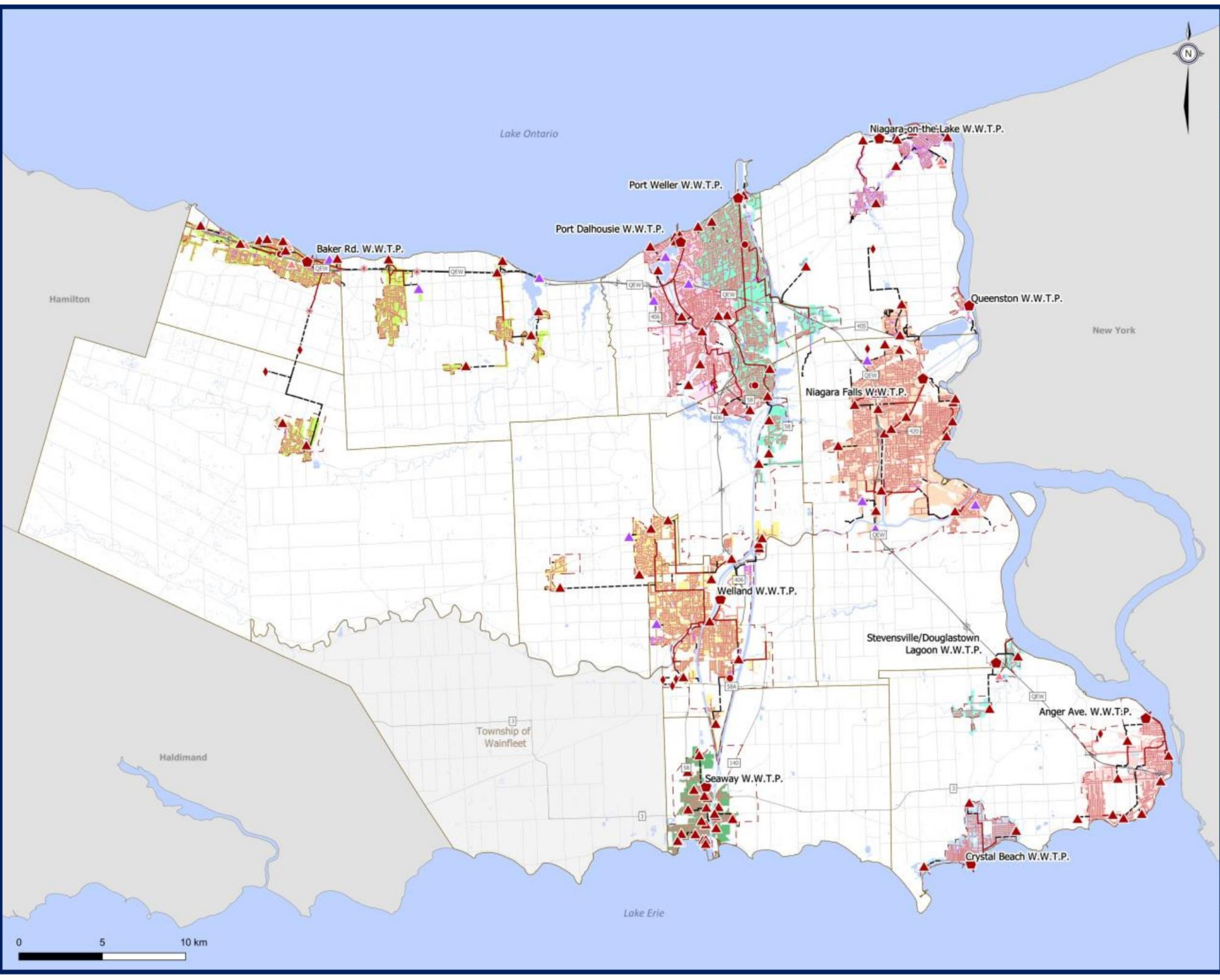
Figure 2.9 Wastewater System Overview Baseline System Understanding
