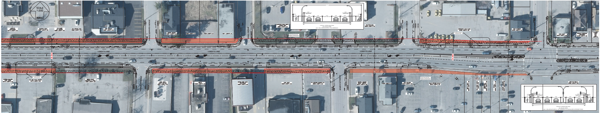
PR 26.20m RIGHT-OF-WAY PREFERRED ALTERNATIVE 3A (1.95m BLVD & 1.8m SWK)
