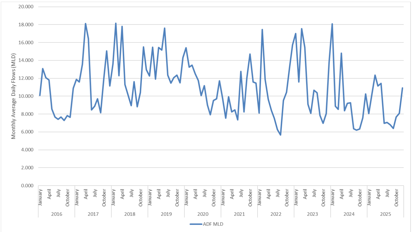
Figure SW-T-1: Graph displaying the Monthly Average Daily Flow Rate in MLD
